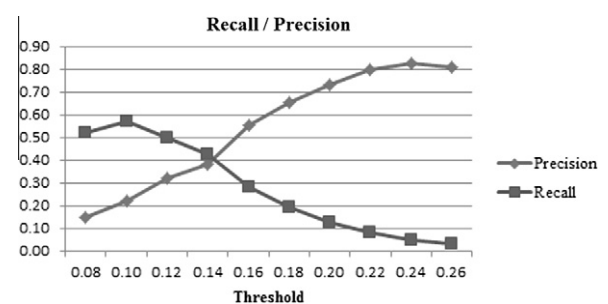
Fig. 6. Precision and Recall when adjusting the threshold.
